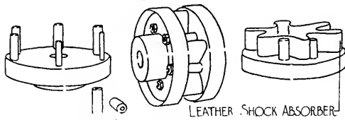
FIG. 235. FLEXIBLE COUPLING.
